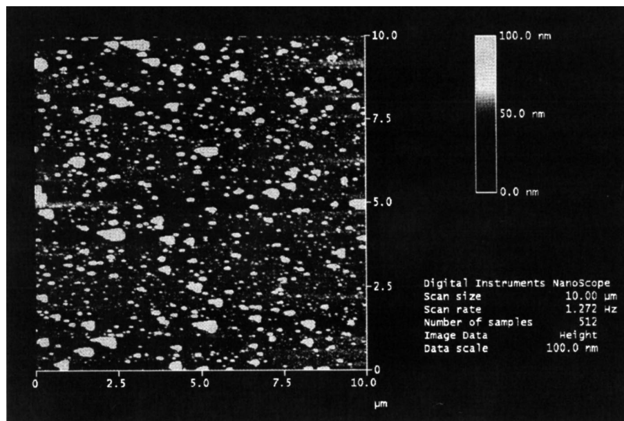
Fig. 27. AFM image of the silver coated ITO surface produced by electrolysis. Figures 26–27 are adopted from [71].
