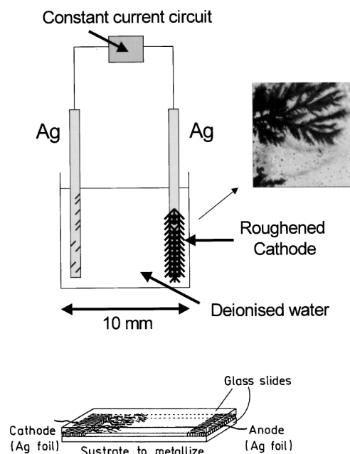
Fig. 28. Constant current apparatus for electrode silver fractal growth (top). Silver growth on glass slide (bottom).
