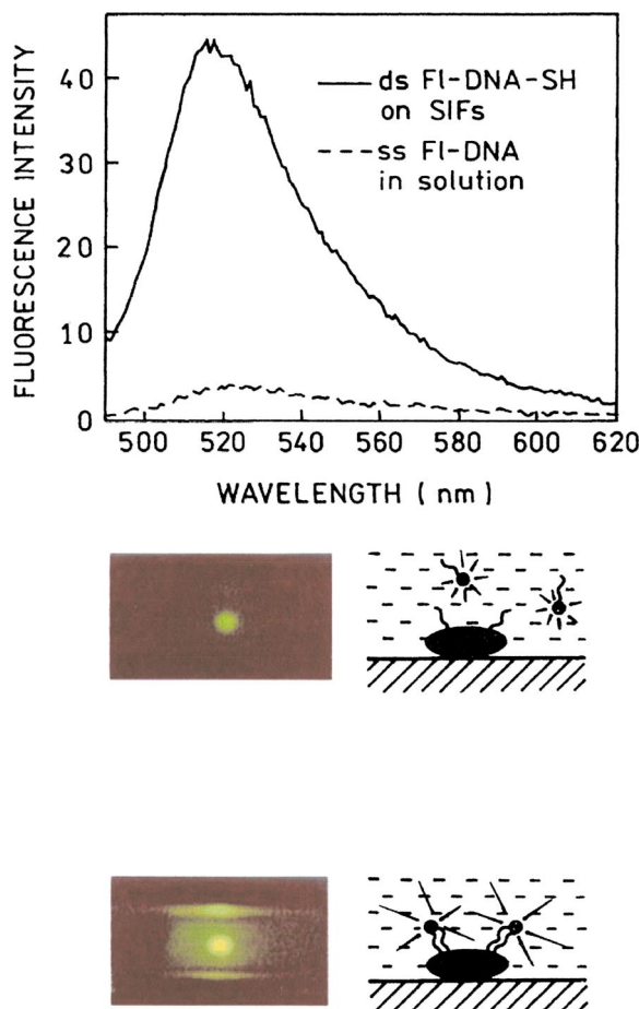
Fig. 16. Emission spectra of ss FI-DNA in solution (dashed line) and bound (solid line) to silver particles. Roughly the same number of molecules of ss FI-DNA and ds FI-DNA-SH was in the illuminated area. The lower panel shows photographs of ss FI-DNA in solution (top) and ds FI-DNA-SH on SIFs (bottom). Figures 14–16 are adopted from [58].
