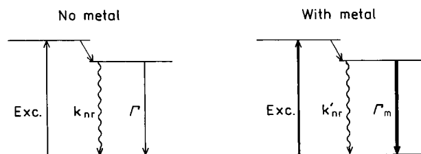
Scheme 1. Jablonski diagram for molecules in absence (left) and presence (right) of metal particles.
