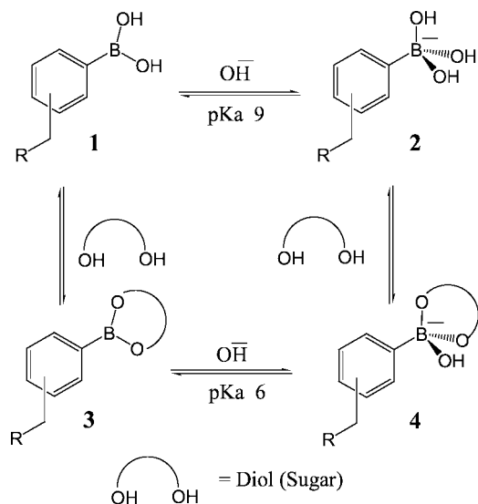
Scheme 1. Equilibrium for the boronic acid/diol (sugar) interaction.
