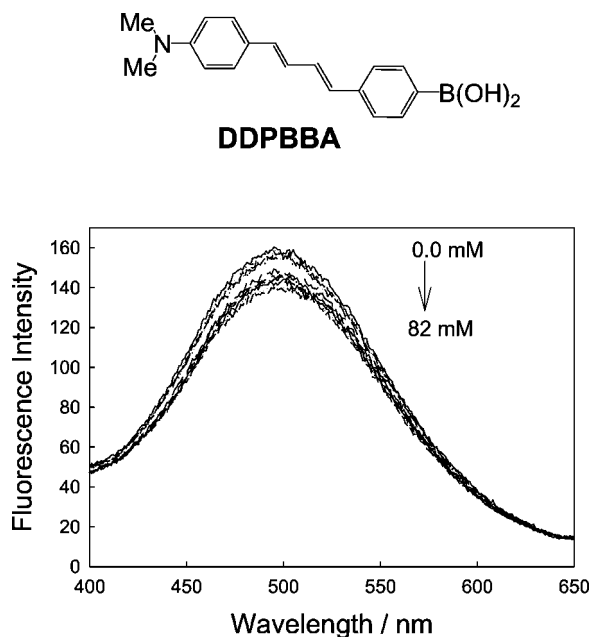
Fig. 3. Molecular structures of the CT probe studied in the contact lens (Top). DDPBBA—1-( p -Boronophenyl)-4-( p -dimethylaminophenyl)buta-1,2-diene. Emission spectra of the DDPBBA doped contact lens, pH 8.0 buffer/methanol (2:1), with increasing concentrations of glucose, \lambda_{\text{ex}} = 340 \text{ nm} (Bottom).
