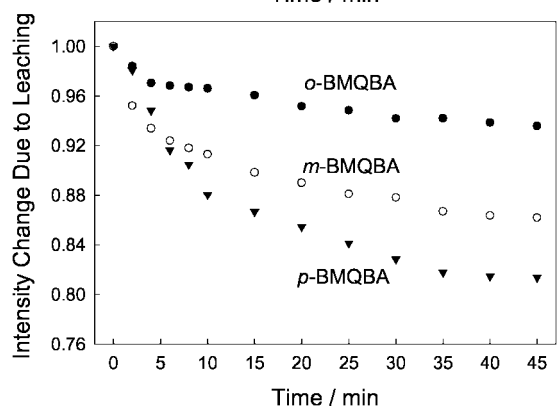
Fig. 15. Emission spectra of o -BMQBA in the lens immersed in pH 7.5 buffer with time (Top). \lambda_{\text{ex}} = 320 nm. Normalized intensity change at band maximum of BMOQBA with time due to leaching (Middle), and that for the BMQBAs (Bottom).
